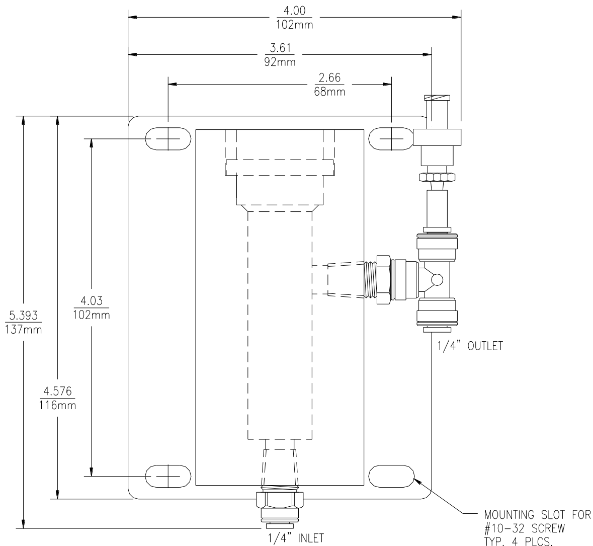
Figure 7 - Fluoride Flowcell
